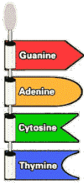
NUCLEOTIDES
